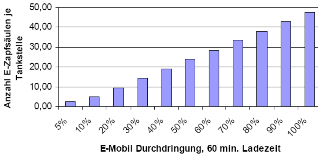
Figure 15. Number of electric fueling facilities per fueling stations in Austria. 40
