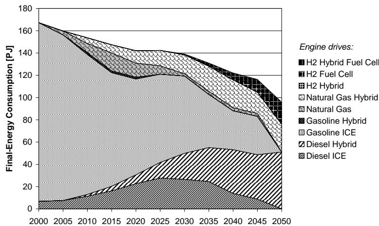
Figure 16. Final-energy consumption of passenger cars at an oil price of 75US 2000 /bbl, 3.5 kW/Cap primary energy and a CO 2 reduction constraint of 10 % per decade. 18
