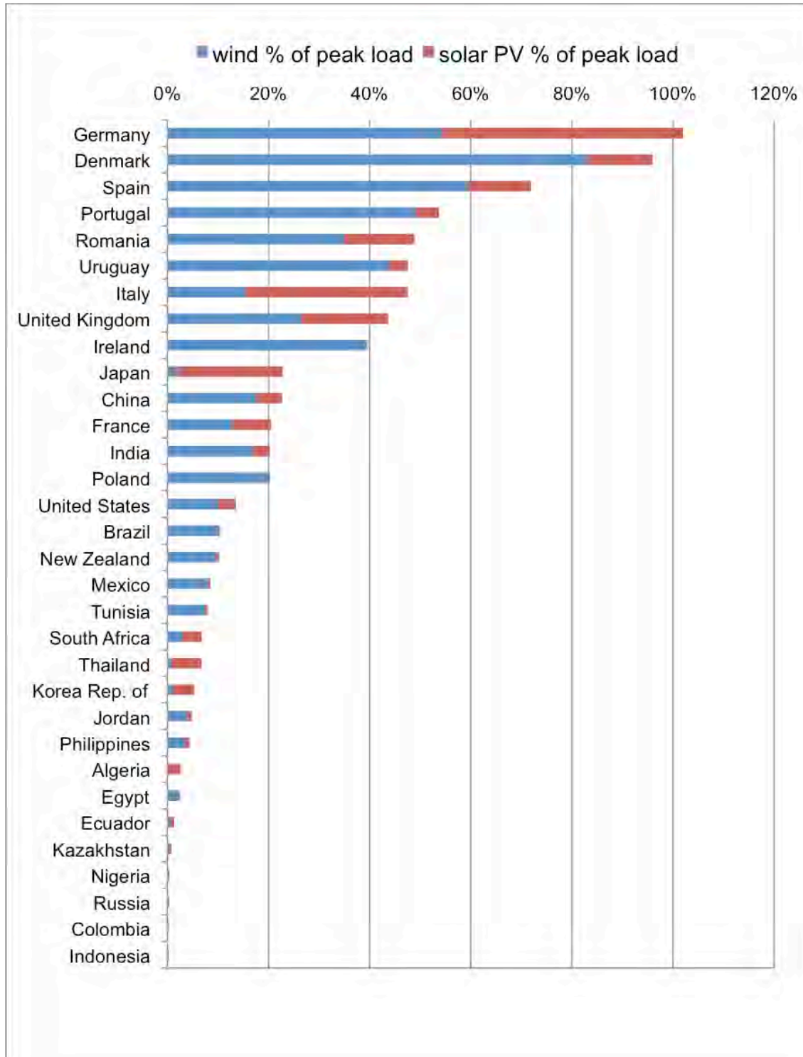
FIGURE 9-2015 VRES CUMULATIVE INSTALLED CAPACITY BY COUNTRY IN PERCENT OF THE NATIONAL PEAK LOAD
